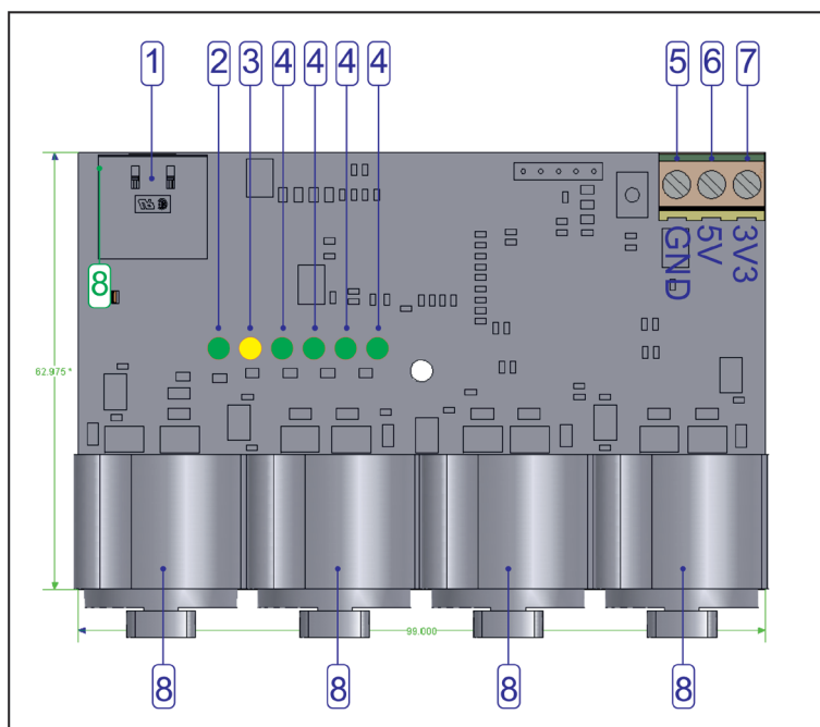
Connections diagram
