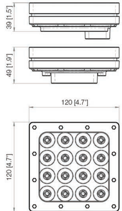
Solaris Mozart FLR Dimensions in MM [inches]
