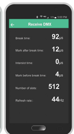
DMX Tester
